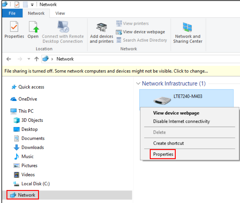
Figure 101 Network Connections
