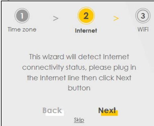
Figure 38 Wizard - Internet
