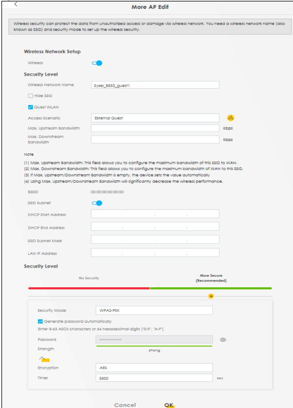
Figure 74 Network Setting > Wireless > More AP Edit
