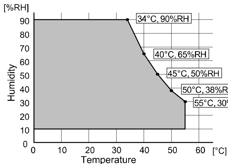
Figure 20-1 Operating Temperature and Humidity Range (Printing)
