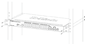
Figure 4. Installing the switch in a standard-sized equipment rack
