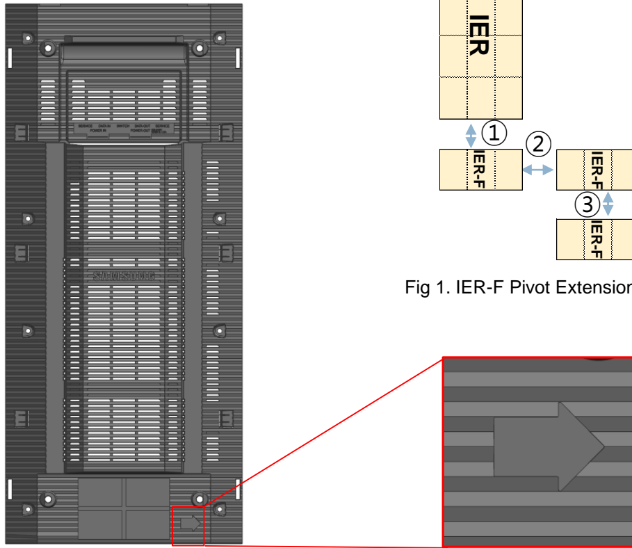
Fig 3. Pivot Arrow on the Rear
