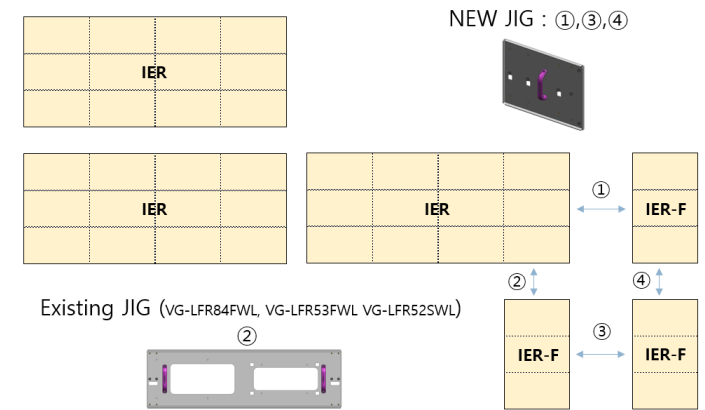
Fig 1. IER-F Extension for General Installation of IER
