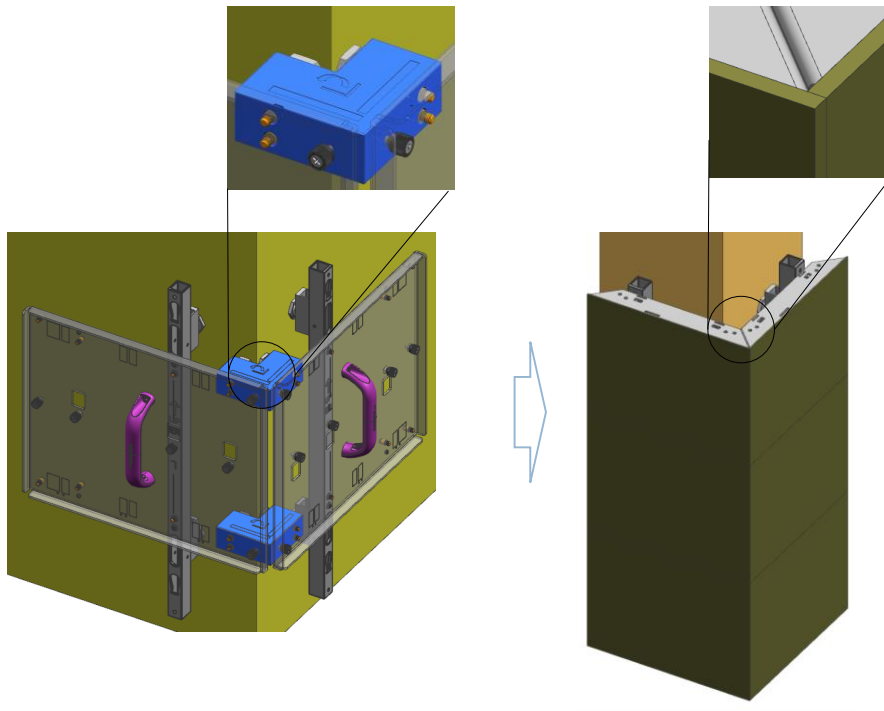
Fig 24. L Support Marks and Module Overlapping Structure
