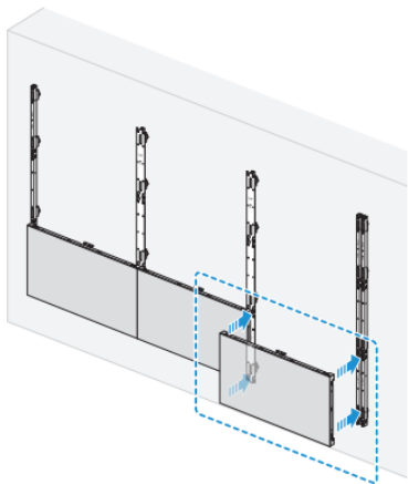
Fig.6 Installing cabinets
