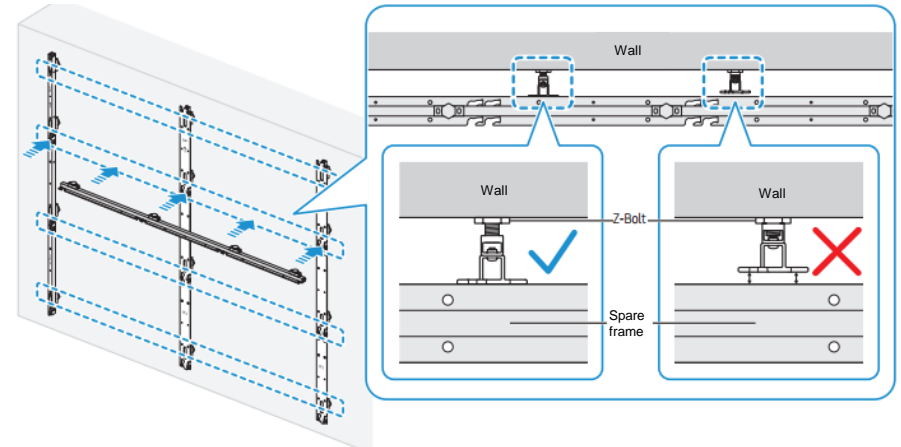
Flatness measurement positions: Around areas where screws are fastened
