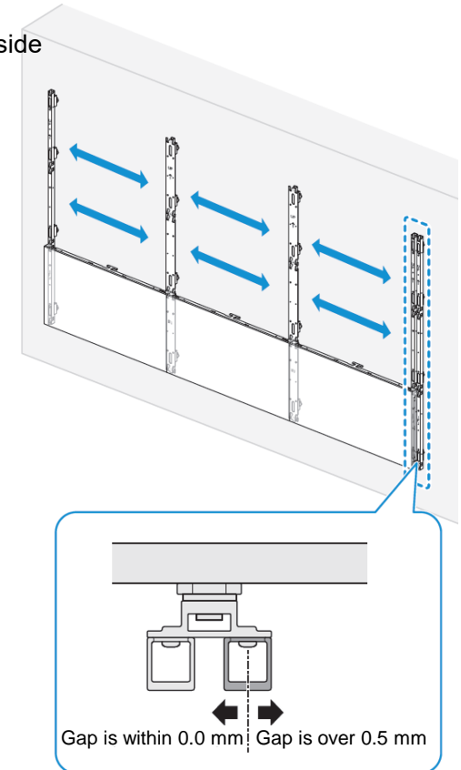
Fig.8 (adjust the gap)
