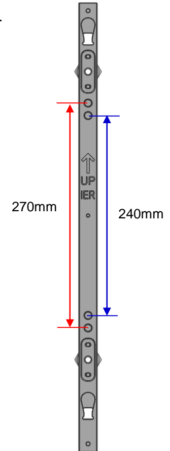
Fig 6. FRAME F JIG HOLE
