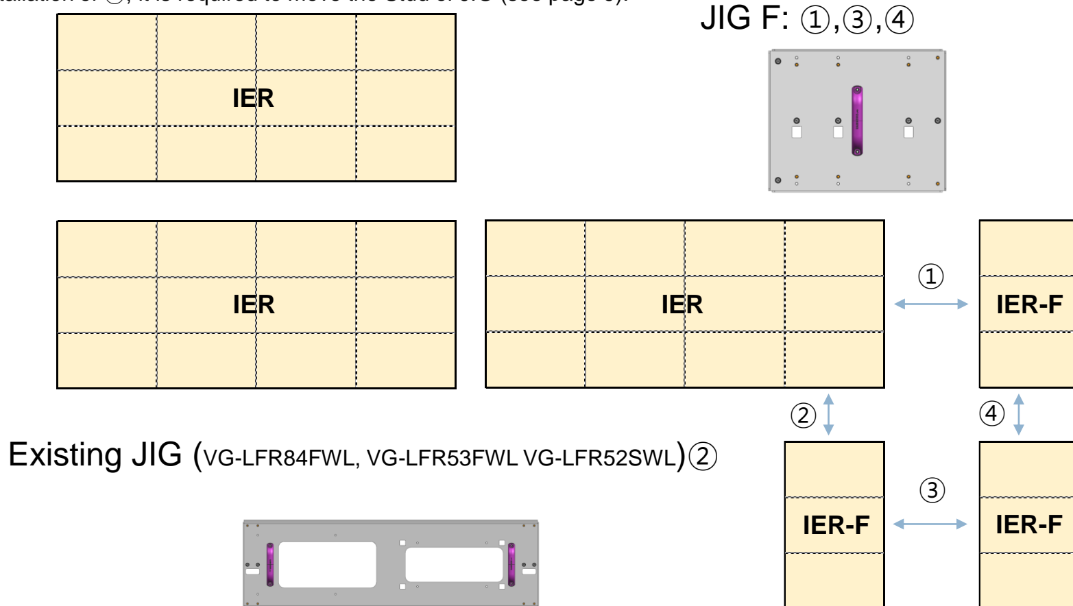
Fig1. IER-F Extension for General Installation of IER
