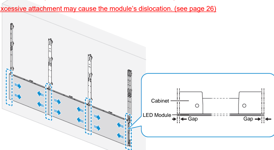
Fig.7 (check the gap)
