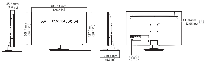
Fig. 1: Dimensions High Performance LED monitor (27 in.)
